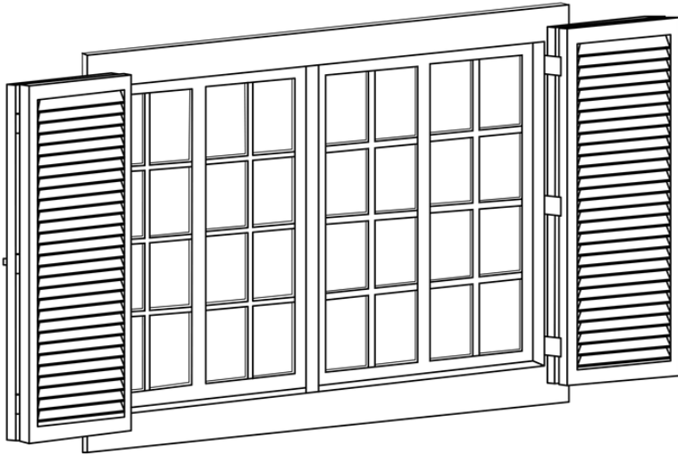
Plan View #5 Louver Side Open 1-1/4" Build Out
