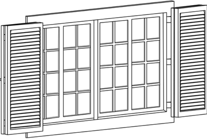
Plan View #8 Louver Side Open 1-1/4" Build Out
