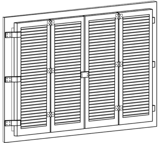
Plan View #5 Flat Side Closed 1-1/4" Build Out
